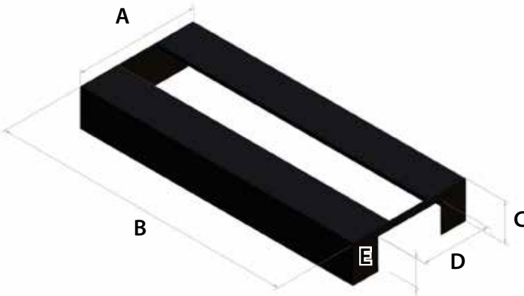
Optional GVF-42 Burner Cover Peninsula
