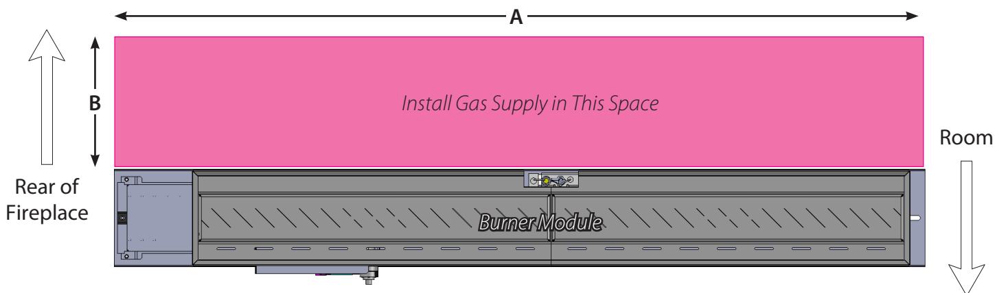
Plan View of Burner Module Showing Gas Supply Area at the Rear
