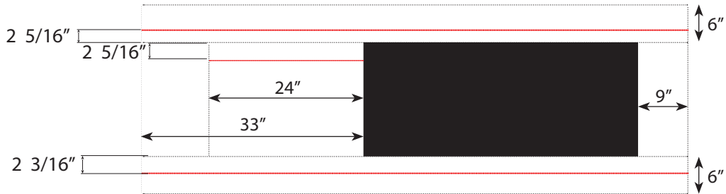
Layout Lines for the Fulcrum 42 (not to scale) (red lines for z-clips)
