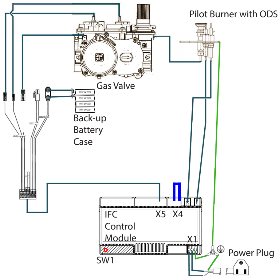
Electric Installation
