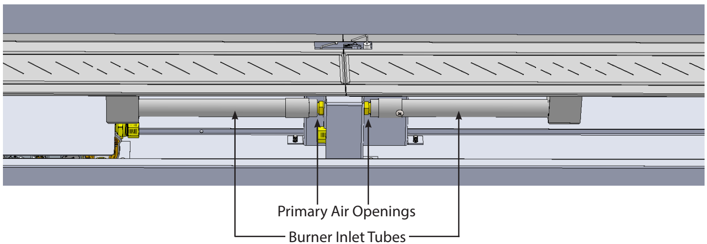
Burner Close-up
