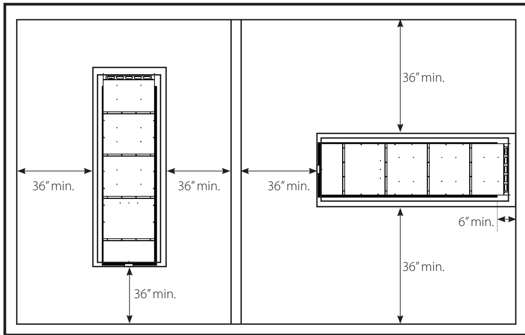
Possible Fireplace Locations (drawing not to scale)
