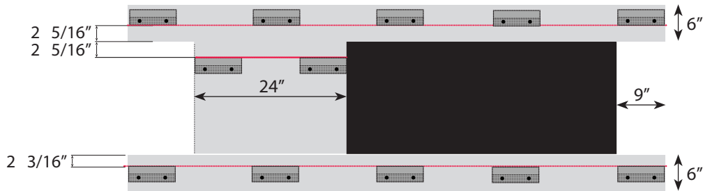
Align Z-Clips to the Red Lines
