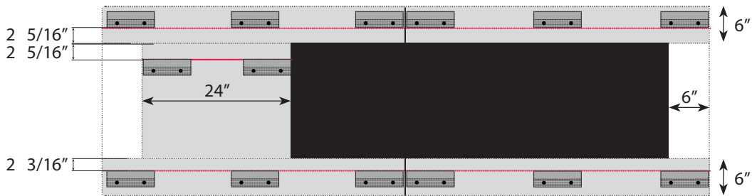
Align Z-Clips to the Red Lines
