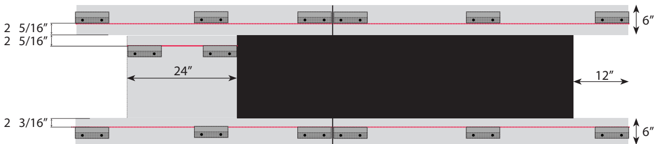
Align Z-Clips to the Red Lines
