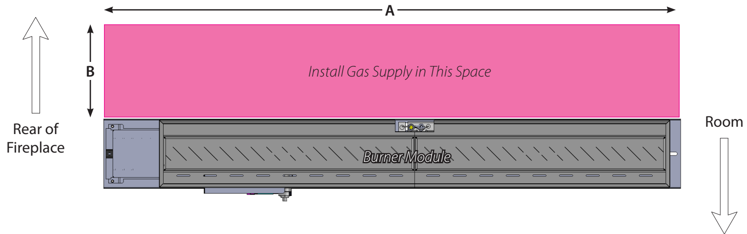
Plan View of Burner Module Showing Gas Supply Area at the Rear
