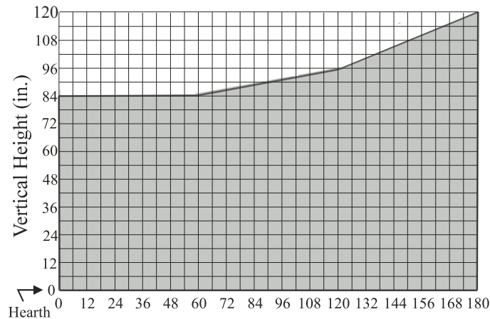
Graph for Top Venting ONLY
